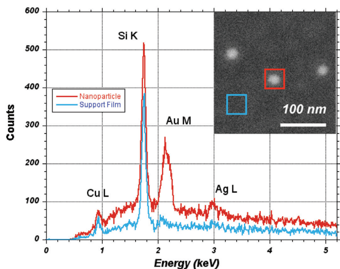
Figure 4: XEDS spectrum (red) obtained from a ~ 20 nm diameter Au nano-particle (inset) compared to the background signal (blue) from the thin SiO 2 support film. The integrated peak intensity of the Au M lines is 2725 counts, acquisition time = 20 live seconds, and the beam current = 0.025 nA at 20 keV. The Cu L and Ag L lines are systems peaks.
